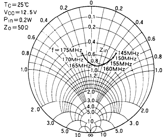
INPUT IMPEDANCE VS. FREQUENCY
