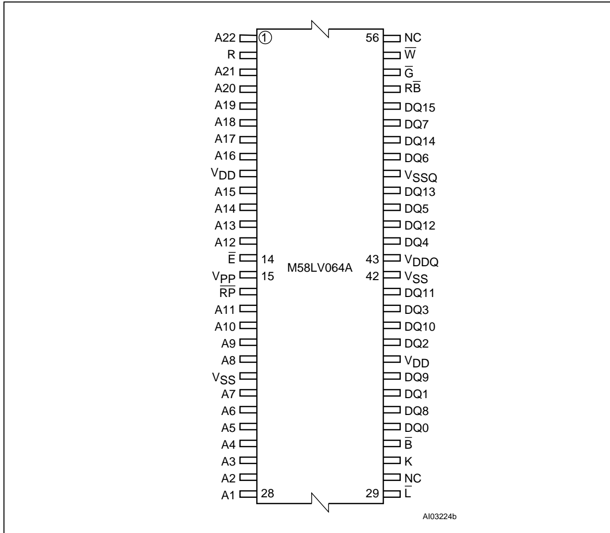
Figure 3. TSOP56 Connections
