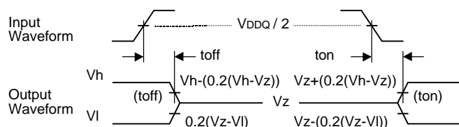
Fig.3 Tri-State measurement
