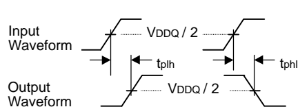
Fig.2 Tdly measurement
