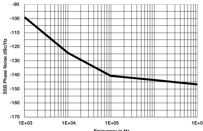
Phase Noise
