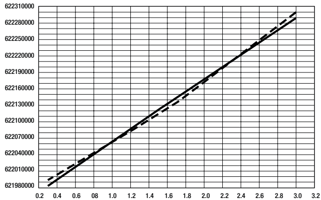
Typical linearity of a M650 operating at 622.08 MHz over the input range of .3 to 3.0 volts
