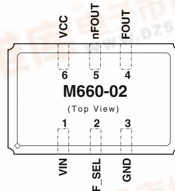
Figure 1: Pin Assignment
