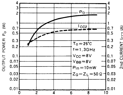
OUTPUT POWER, 2nd CURRENT VS. 1st SUPPLY VOLTAGE CHARACTERISTICS
