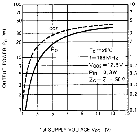
OUTPUT POWER, 2nd CURRENT VS. 1st SUPPLY VOLTAGE CHARACTERISTICS
