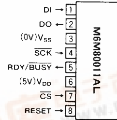
Outline 8P5K
