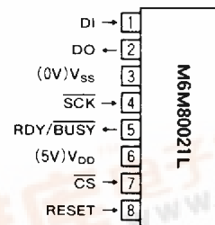
Outline 8P5K
