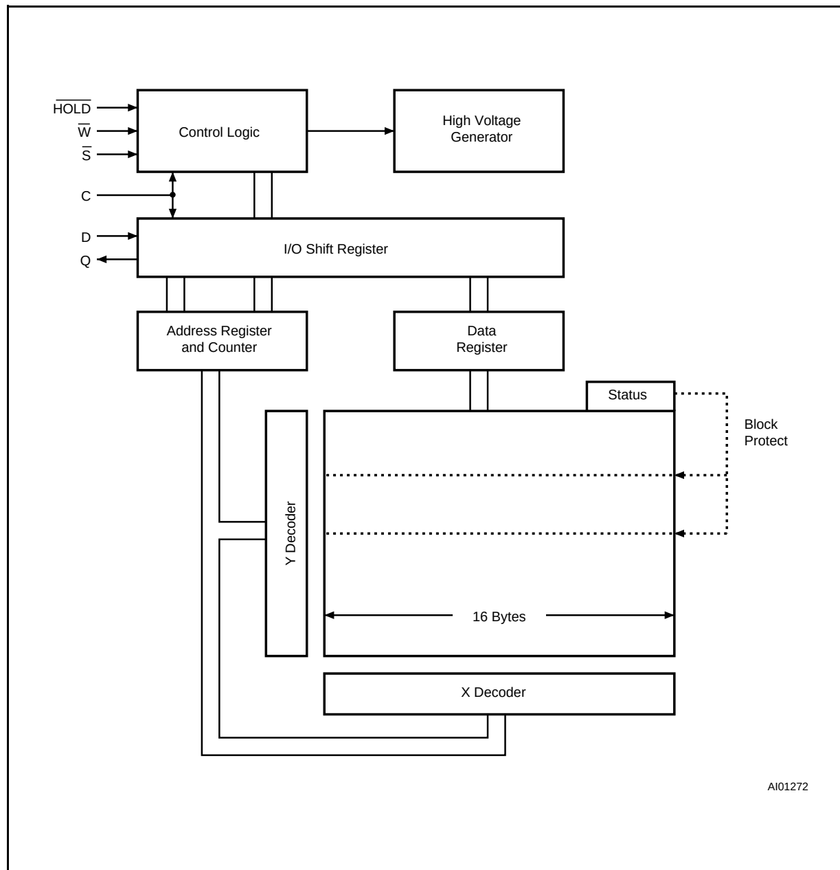
Figure 3. Block Diagram
