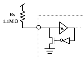
Fig.1 Encoder Oscillator
