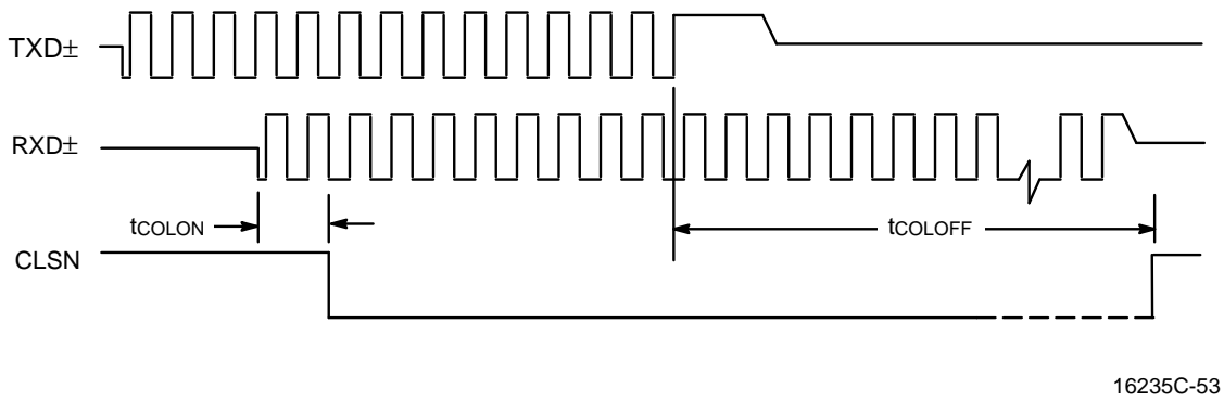
10BASE-T Collision Timing
