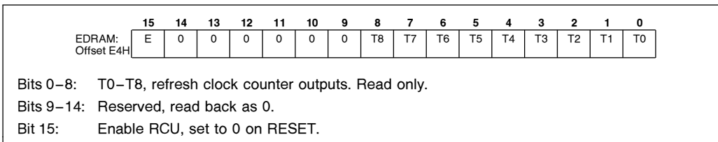
Figure 43. Enable RCU Register
