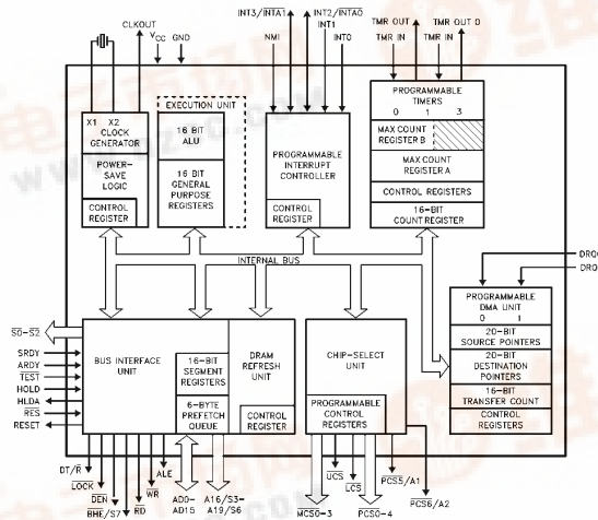
Figure 1. M80C186 Block Diagram
