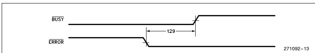
Figure 15. ERROR Output Timing
