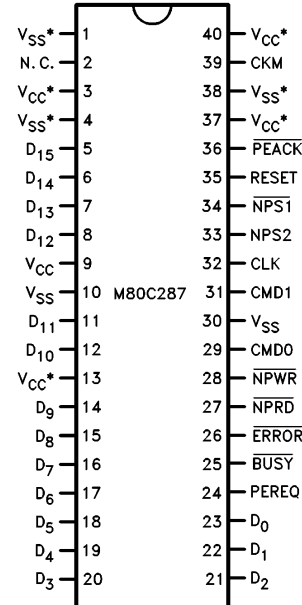
Figure 8. Cerdip Pin Configuration
