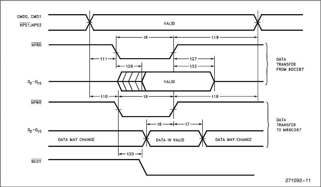
Figure 13. Data Transfer Timing (Initiated by CPU)
