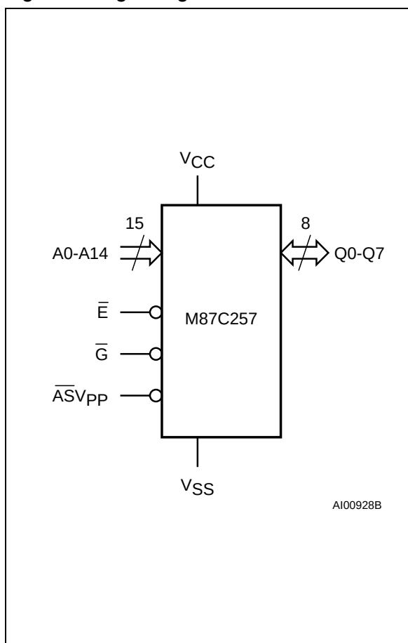
Figure 1. Logic Diagram
