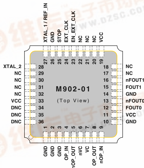
Figure 1: Pin Assignment
