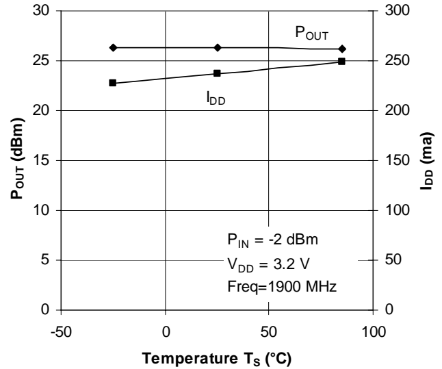
Figure 6. Output power and drain current vs. temperature at V_{DD}=+3.2V
