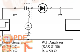
Bias Application Unit N-50BU
