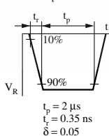
Input Pulse
