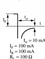
Output Pulse
