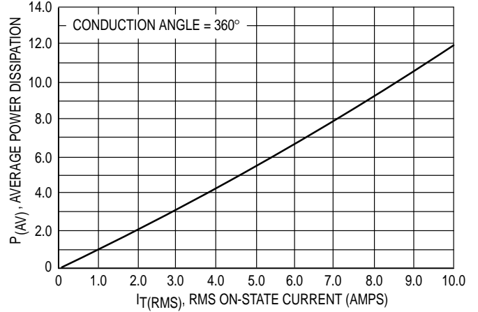
FIGURE 2 — POWER DISSIPATION
