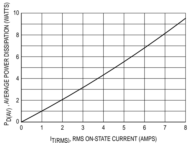
Figure 2. Power Dissipation
