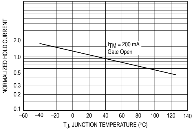
FIGURE 5 – HOLDING CURRENT
