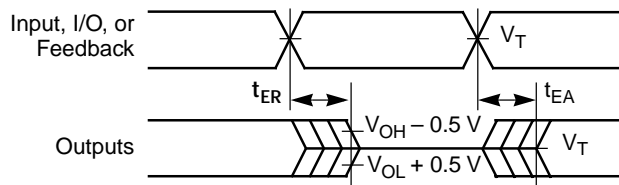
Output Disable/Enable
