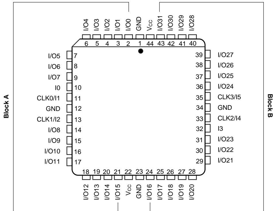
44-Pin PLCC
