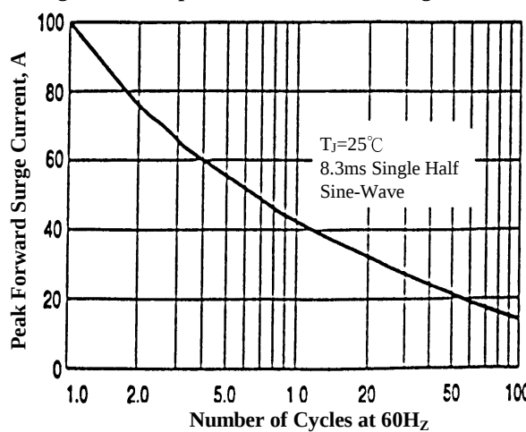
Fig. 4 - Non-Repetitive Peak Forward Surge Current
