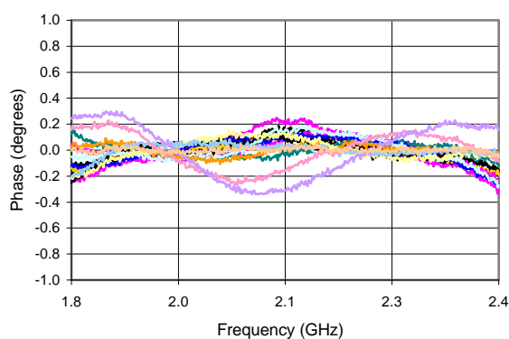
Phase vs. Frequency
