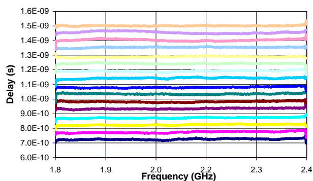
Delay vs. Frequency
