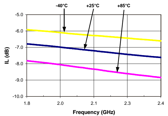
Insertion Loss vs. Frequency over Temperature at 750 pS State
