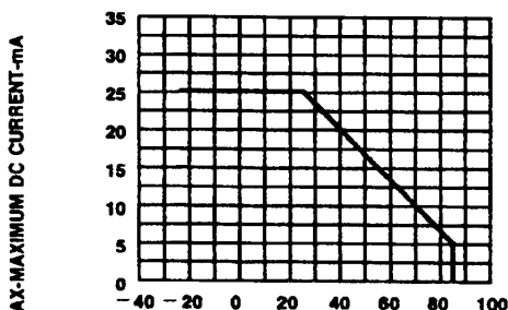
T_A AMBIENT TEMPERATURE ^\circ\text{C} Fig.4 MAXIMUM ALLOWABLE DC CURRENT PER SEGMENT CS. A FUNCTION OF AMBIENT TEMPERATURE.
