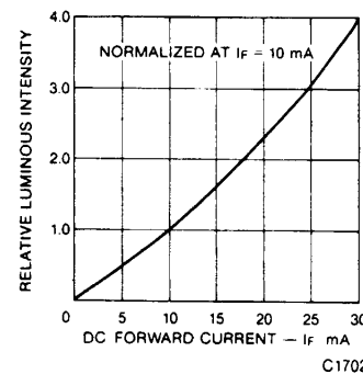
Fig. 6. Relative Luminous Intensity vs. Forward Current
