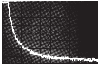
Figure 8. Low Frequency Noise Spectrum Showing Low 2 Hz Noise Corner, Gain = 1000
