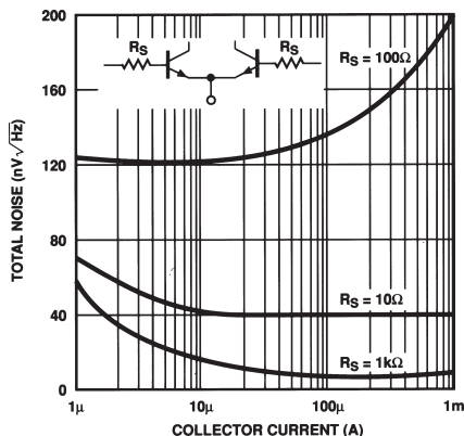
TPC 10. Total Noise vs. Collector Current
