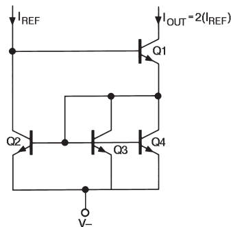
Figure 2. Current Mirror, I_{OUT} = 2(I_{REF})
