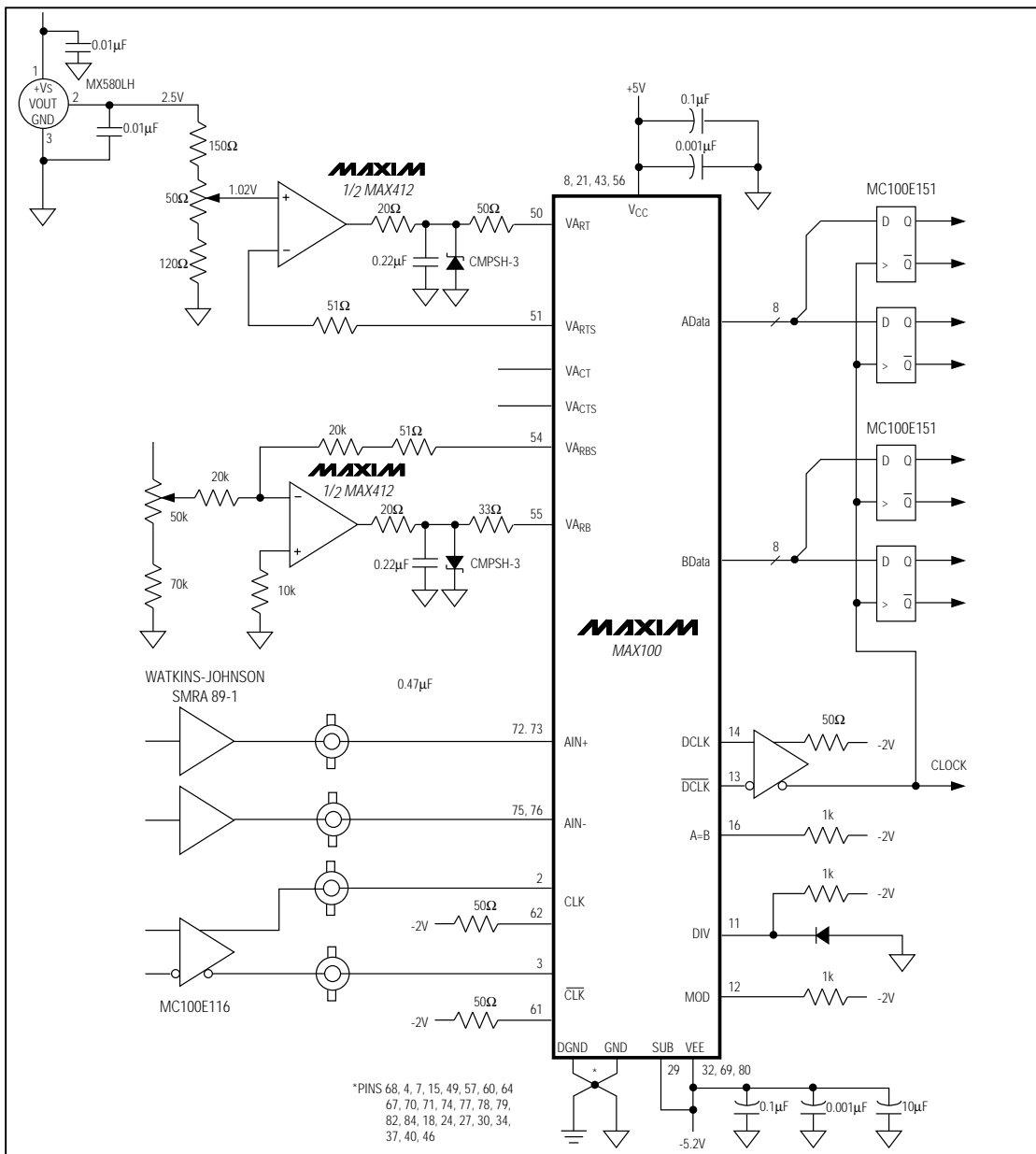
Typical Operating Circuit
