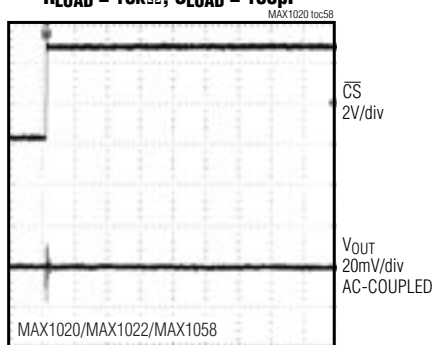
MAJOR CARRY TRANSITION R_{LOAD} = 10k\Omega , C_{LOAD} = 100pF
