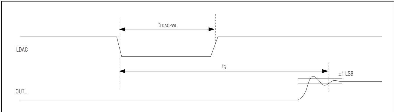
Figure 14. LDAC Functionality
