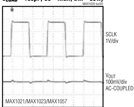
DAC DIGITAL FEEDTHROUGH ( R_{LOAD} = 10k\Omega , C_{LOAD} = 100pF , CS = HIGH, DIN = LOW)
