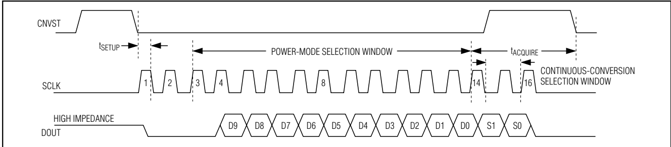
Figure 5. Interface-Timing Sequence
