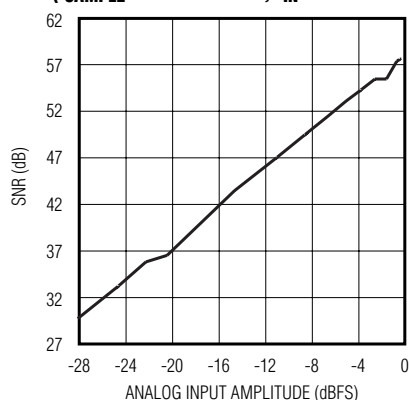
SNR vs. ANALOG INPUT AMPLITUDE ( f_{SAMPLE} = 210.0057MHz , f_{IN} = 60.0126MHz )
