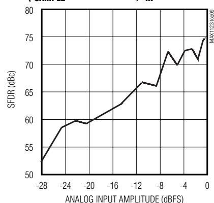
SFDR vs. ANALOG INPUT AMPLITUDE ( f_{SAMPLE} = 210.0057MHz , f_{IN} = 60.0126MHz )
