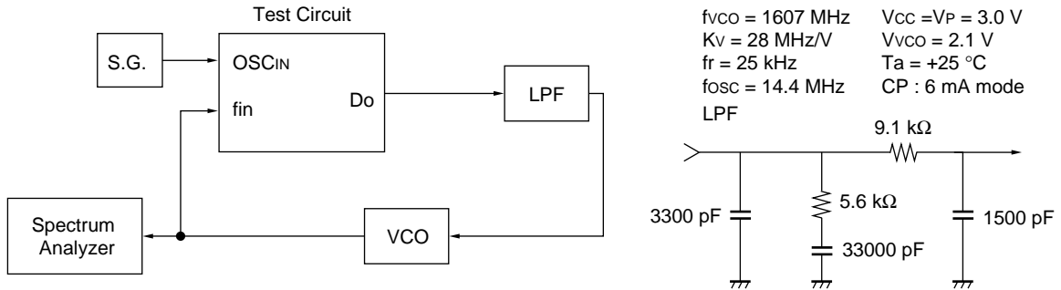
PLL Reference Leakage
