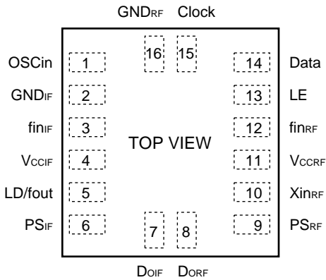
(LCC-16P-M03)
