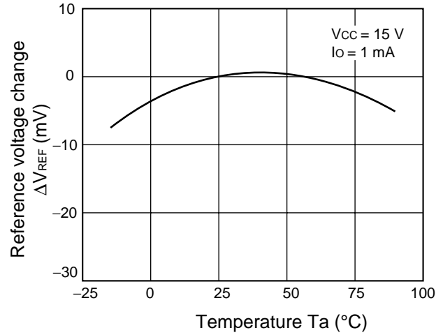
Reference voltages. temperature
