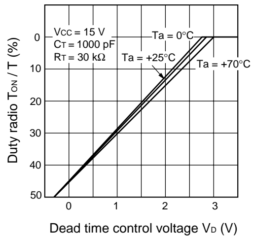
Duty ratio vs. dead time control voltage
