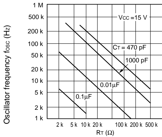
Oscillator vs. R_T , C_T
