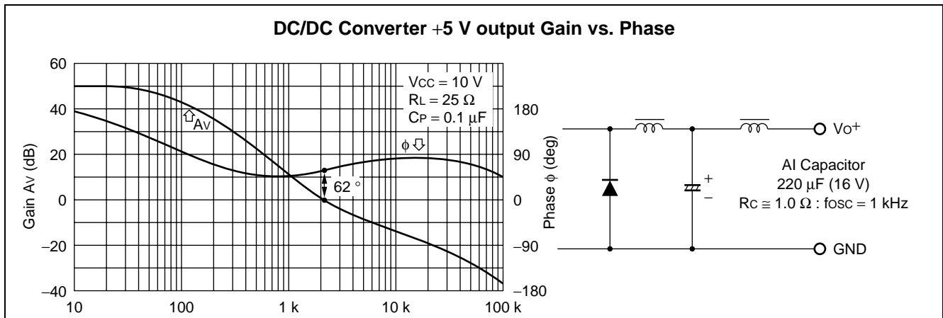
Figure 38 DC/DC Converter +5 V output Gain vs. Phase
