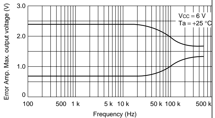
Error Amp. Max. output voltage vs. Frequency
