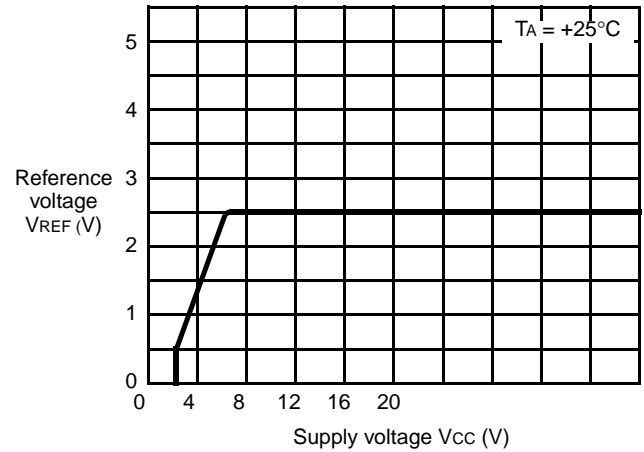
2. Reference voltage - supply voltage characteristic
