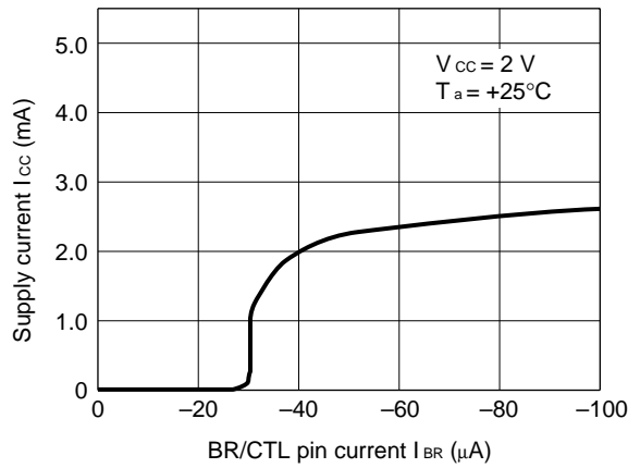
BR/CTL pin current vs. Supply current
