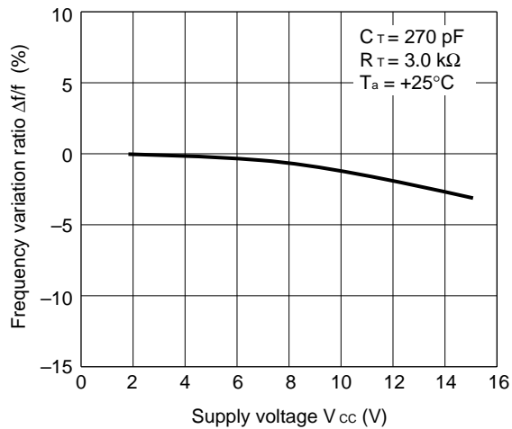
Supply voltage vs. Frequency variation ratio
