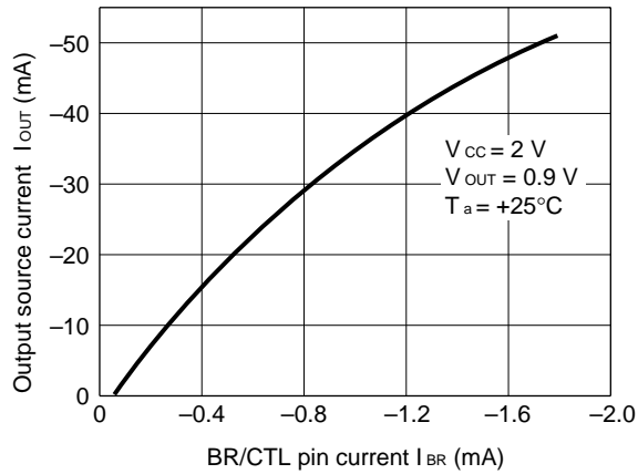
BR/CTL pin current vs. Output source current
