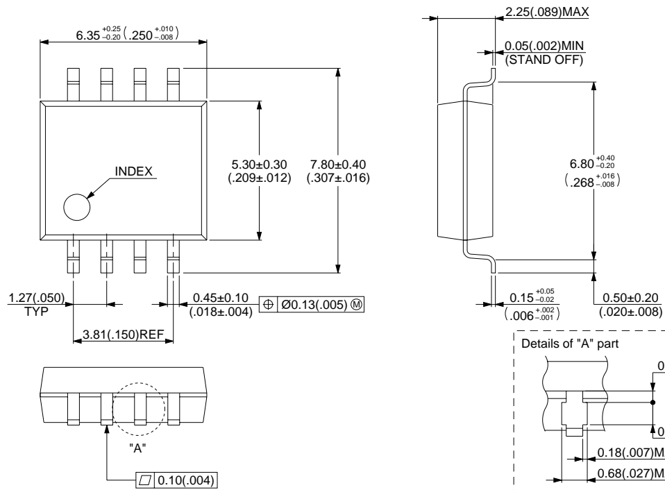
8-pin Plastic SOP (FPT-8P-M01)
