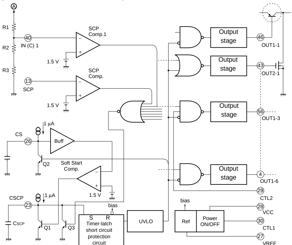
Figure 6. Protection timer-latch short protection circuit
