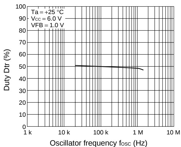
Duty vs. oscillator frequency (ch4)
