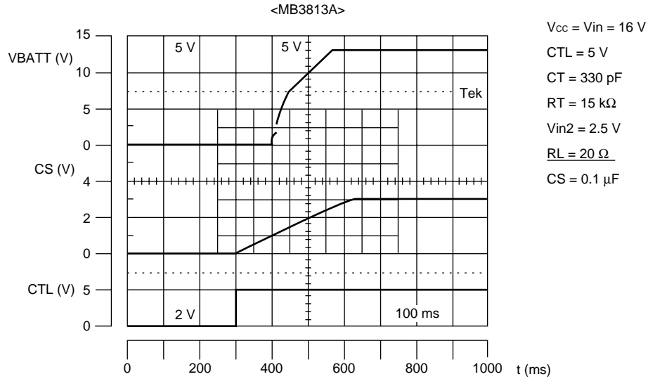
Soft start operation waveforms
