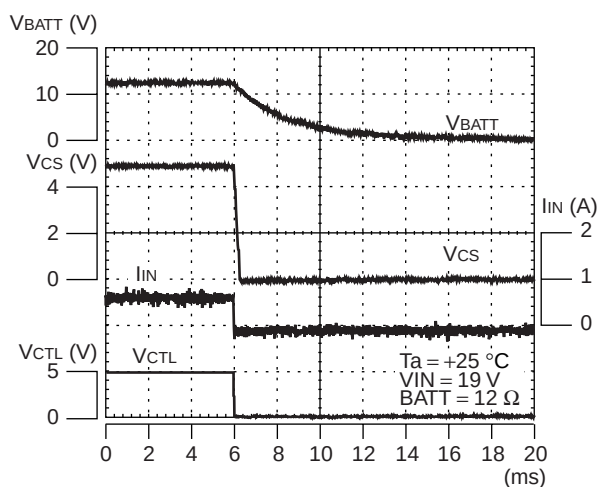
Discharge operating waveform constant voltage mode (set at 12.6 V)
