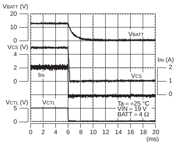
Discharge operating waveform constant current mode (set at 12.6 V)
