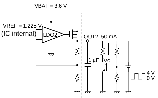
[Measurement diagram]
