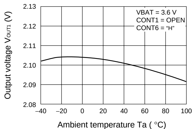
Output voltage vs. ambient temperature (LDO1)
