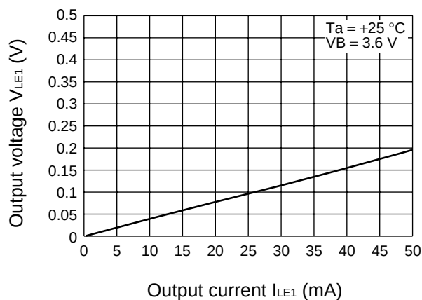
LED1 output voltage vs. output current
