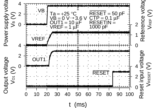
Hold time for power-on-reset
