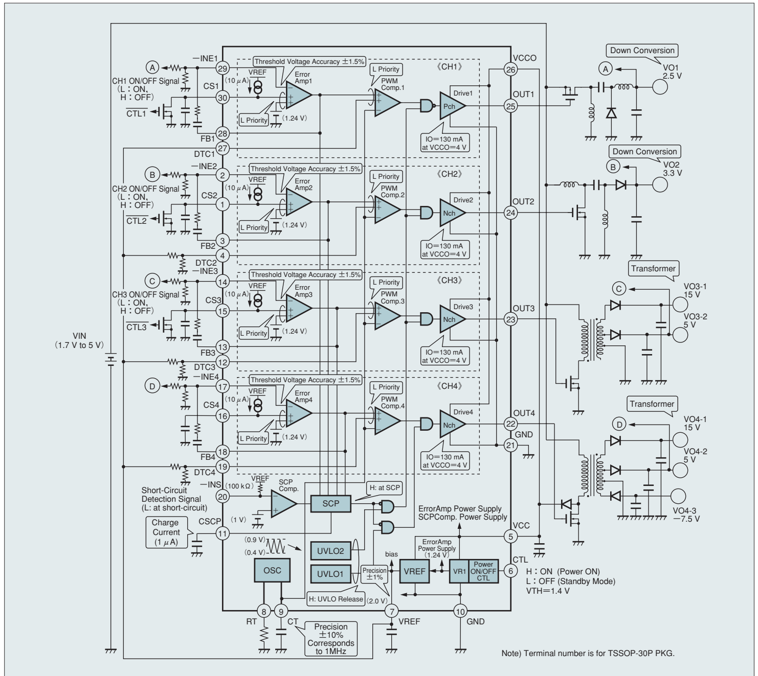
Figure 3 Block Diagram
