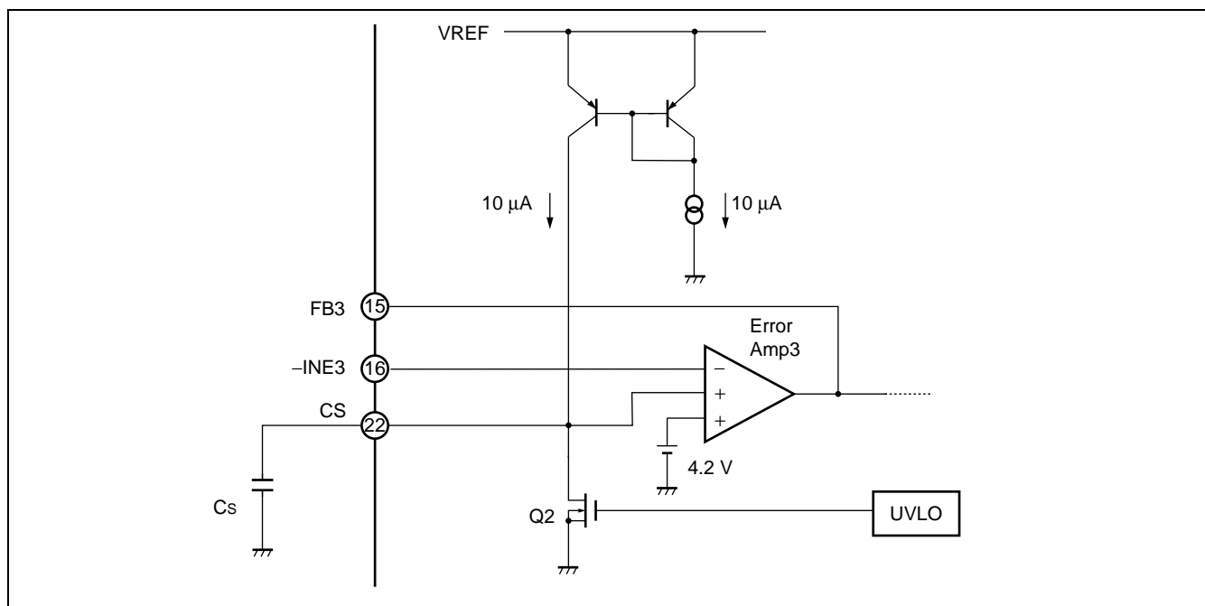
Soft-start circuit
