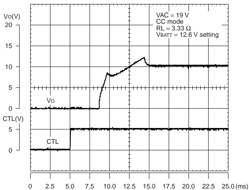
Soft-start Operating Waveform at Constant Current Mode (12.6 V setting) (1)
