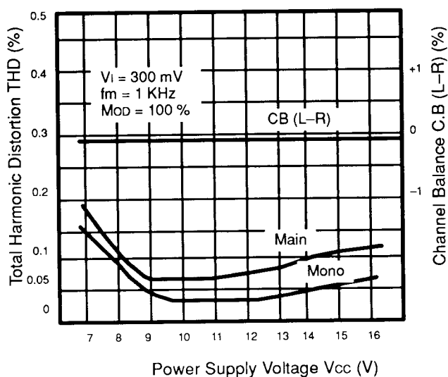
Figure 5 TOTAL HARMONIC DISTORTION (MAIN and MONO), C.B. vs POWER SUPPLY VOLTAGE
