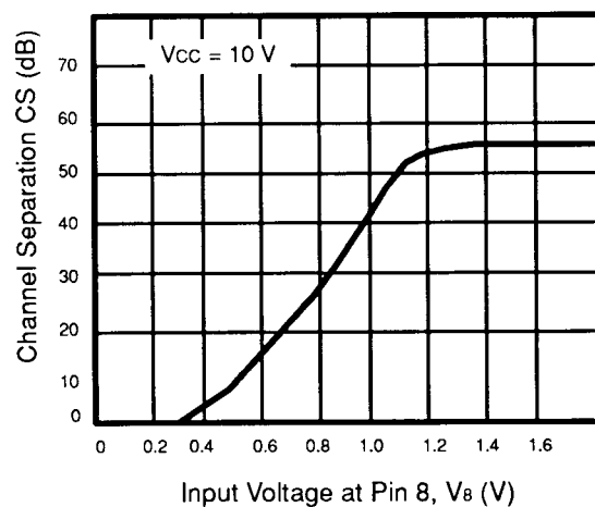
Figure 10 CHANNEL SEPARATION vs INPUT VOLTAGE AT PIN 8
