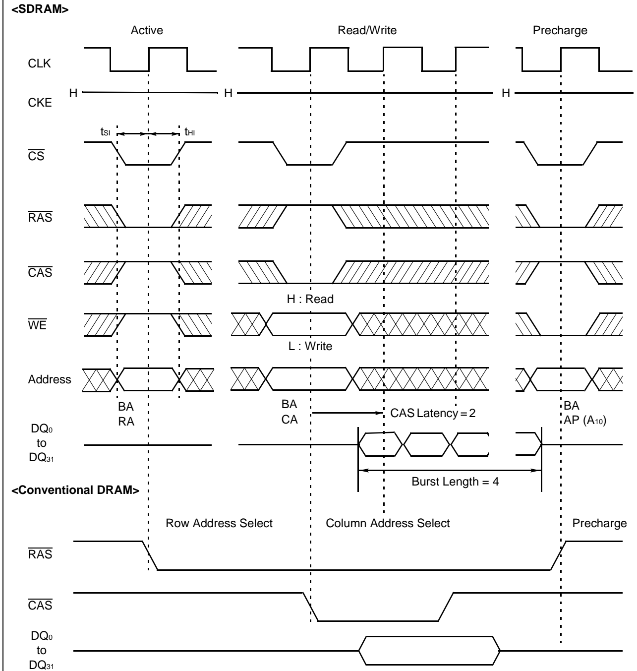
Fig. 2 – BASIC TIMING FOR CONVENTIONAL DRAM VS SYNCHRONOUS DRAM
