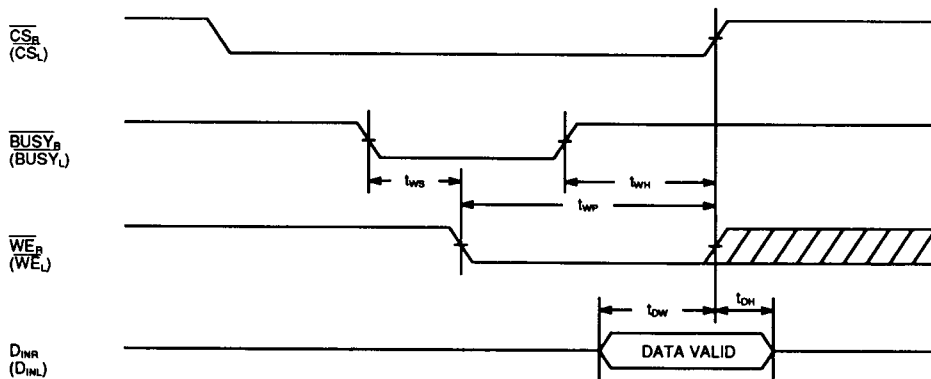
CONTENTION WRITE CYCLE No. 2 *3 : *1 *2 *3 ( \overline{CS} CONTROLLED)
