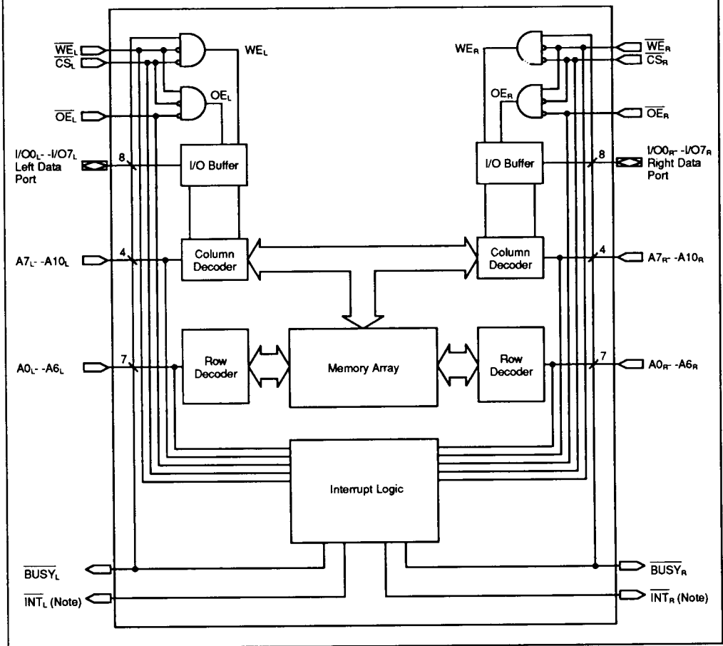
Fig. 1 — MB8431/32/31L/32L BLOCK DIAGRAM
