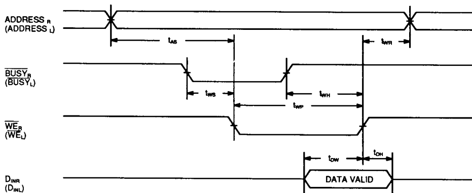
CONTENTION WRITE CYCLE No. 1 *1 *2 *3 ( \overline{WE} CONTROLLED)
