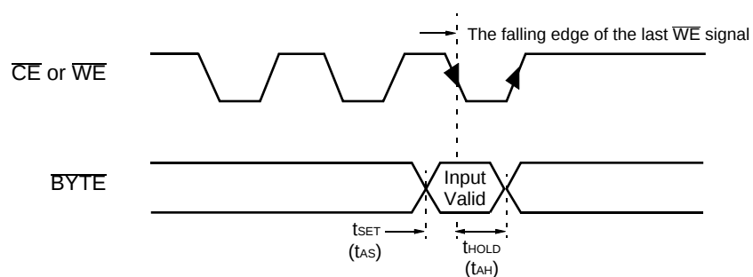
Figure 12 \overline{BYTE} Timing Diagram for Write Operations
