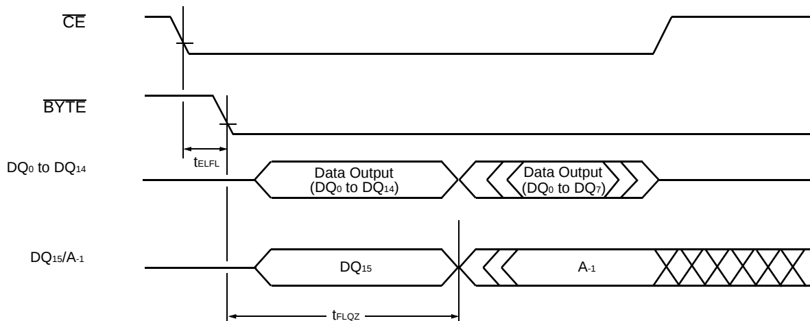
Figure 11 Timing Diagram for Byte Mode Configuration
