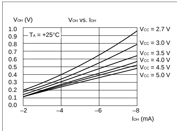
(1) "H" Level Output Voltage
